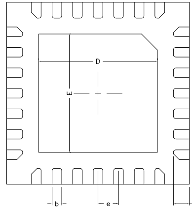
BOTTEM VIEW
