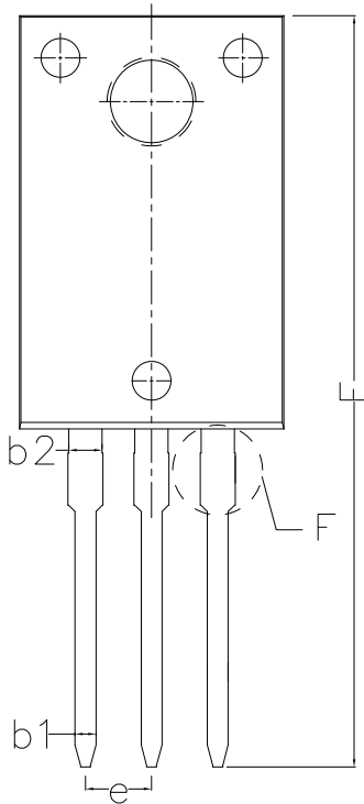
BOTTOM VIEW
