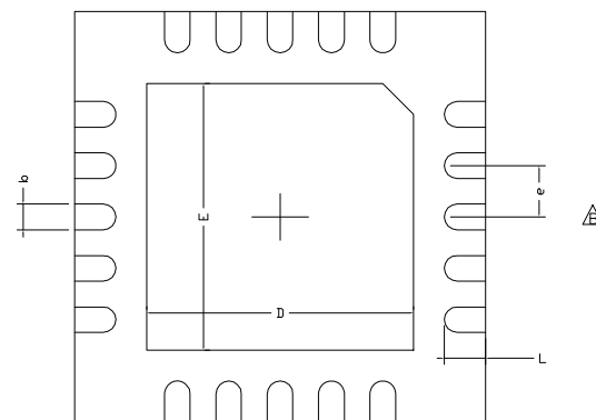
BOTTEM VIEW
